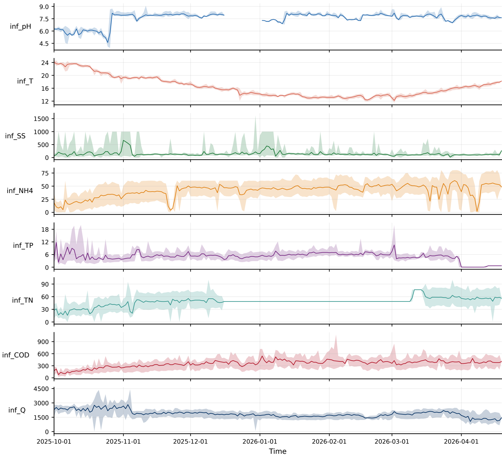
Influent water-quality variables — full-span overview (daily min-max envelope) [2025-10-01~2026-04-19]
